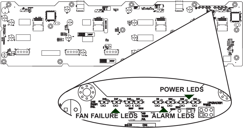
Figure 2-3. Front LEDs
