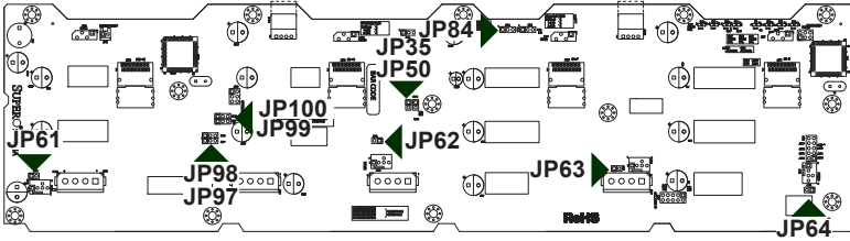
Figure 2-2. Front Jumpers
