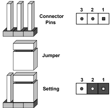
Figure 2-2. Front Jumpers
