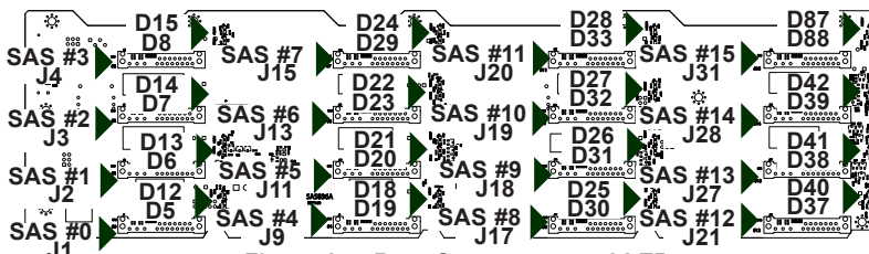
Figure 2-4. Rear Connectors and LEDs
