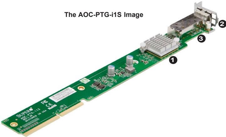
The AOC-PTG-i1S Layout
