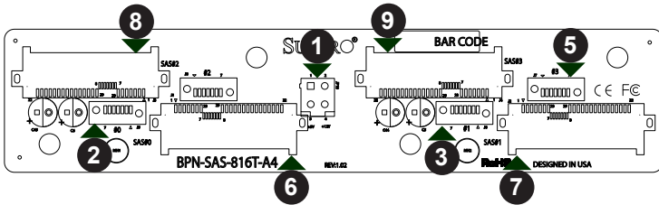
Figure 2-1: Front Connectors
