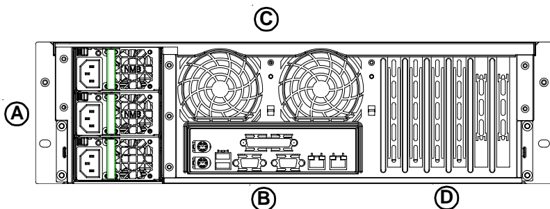
SC933 Chassis Rear View
