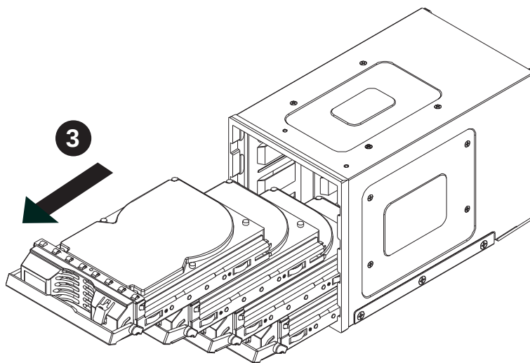
Figure 1-3: Removing the Drives
