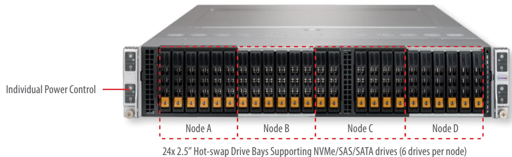
Figure 2. Front View of 2U BigTwin Server System (All-Flash NVMe Model)
