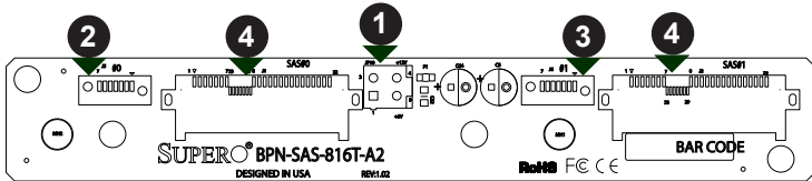
Figure 2-1: Front Connectors
