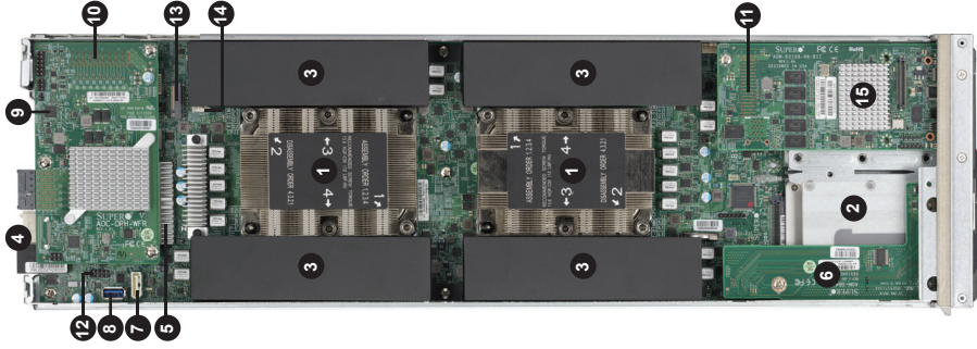
SBI-4129P-T2N/C2N Module Layout
