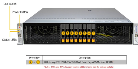
(Front View – System)
