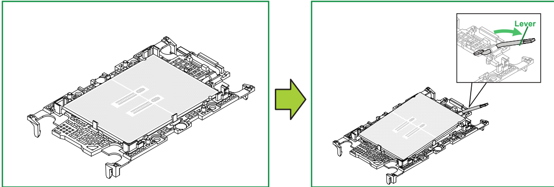
Processor Carrier Assembly (Carrier E1A)
