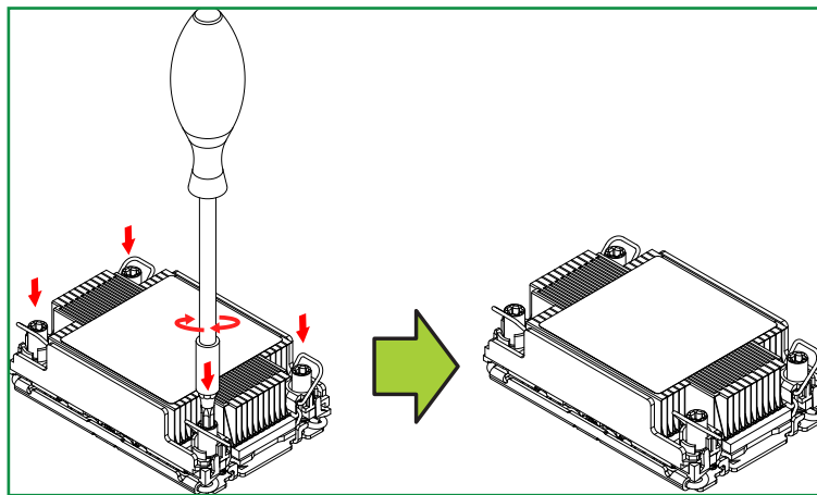
1U Heatsink
