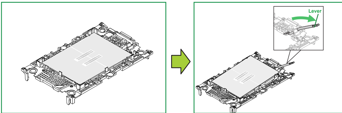
Processor Carrier Assembly (Carrier E1B)
