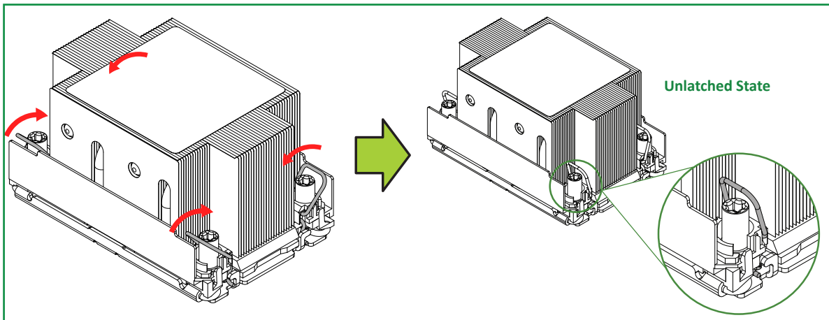
2U Heatsink
