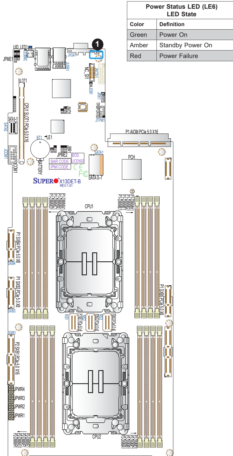
1. Power Status LED (LE6)
