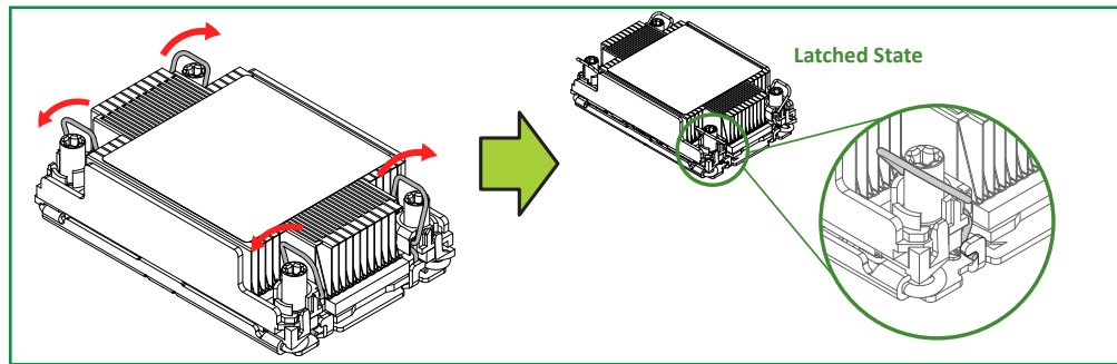
1U Heatsink
