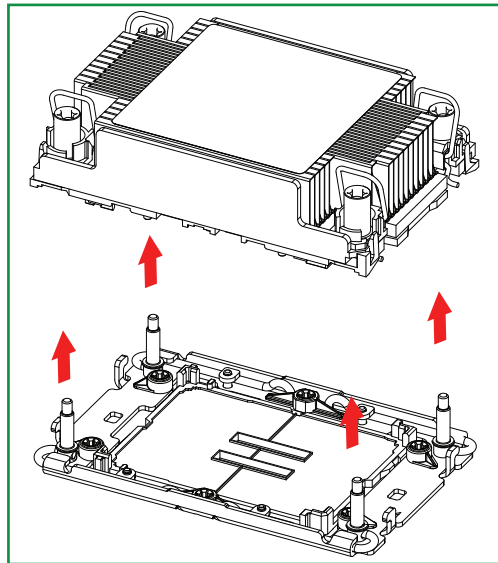
1U Heatsink
