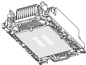
1U Heatsink
