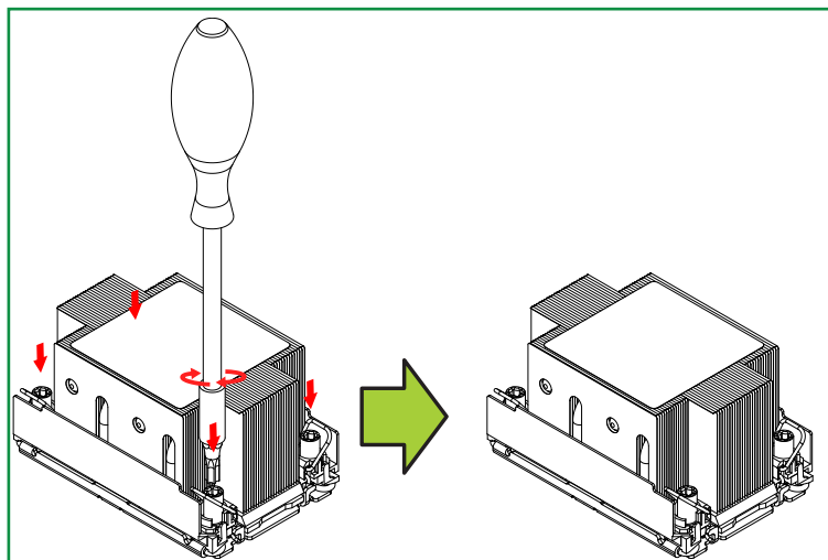
2U Heatsink
