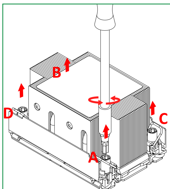
2U Heatsink
