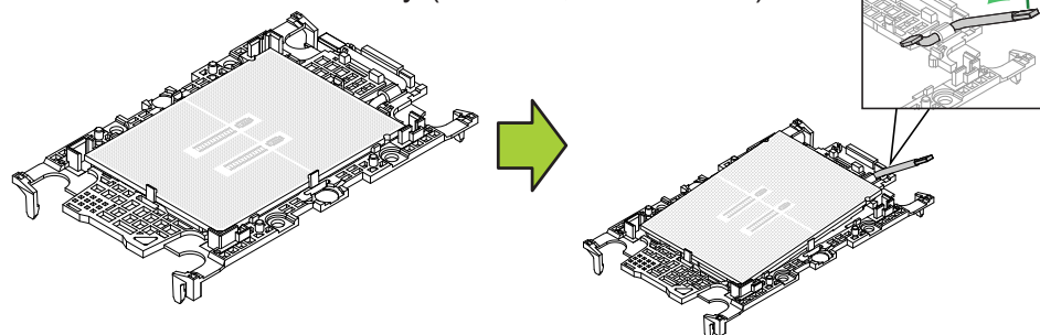
Processor Carrier Assembly (SP XCC, Carrier E1A)
