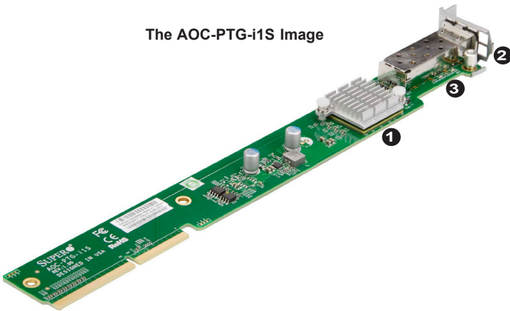
The AOC-PTG-i1S Layout
