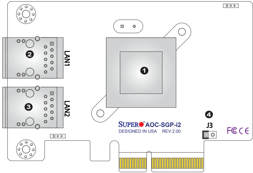
AOC-SGP-i2 Layout
