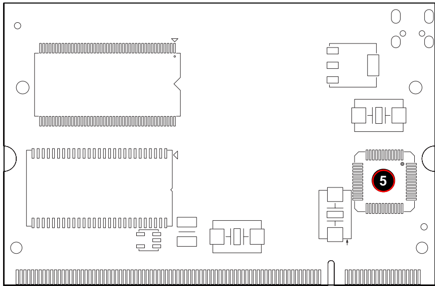
Figure 2-2. AOC-SIMBL Add-on Card – Rear View
