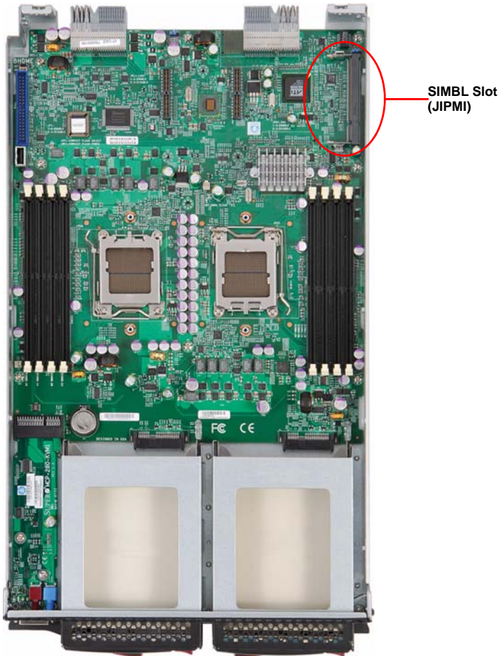
Figure 2-4. Location of SIMBL Slot on BHDME Motherboard
