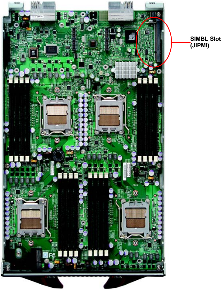
Figure 2-5. Location of SIMBL Slot on BHQIE Motherboard
