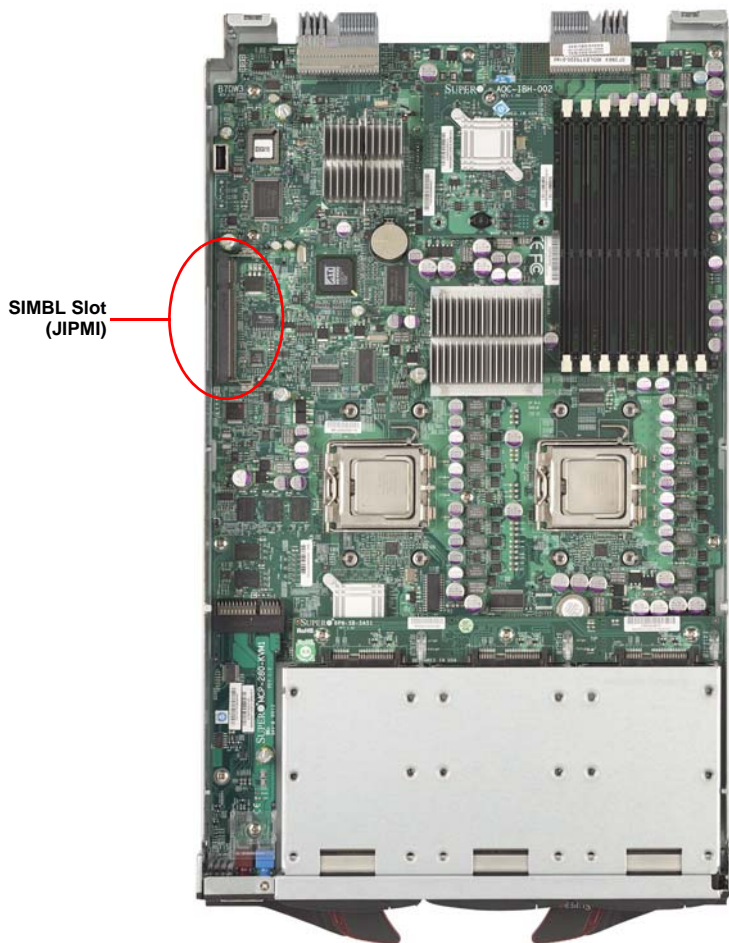
Figure 2-8. Location of SIMBL Slot on B7DW3 Motherboard
