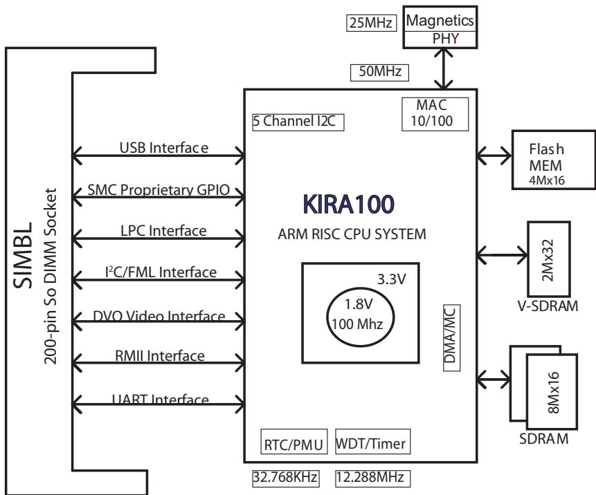
The block diagram for the AOC-SIMBL add-on card is shown in Figure 2-3 .
