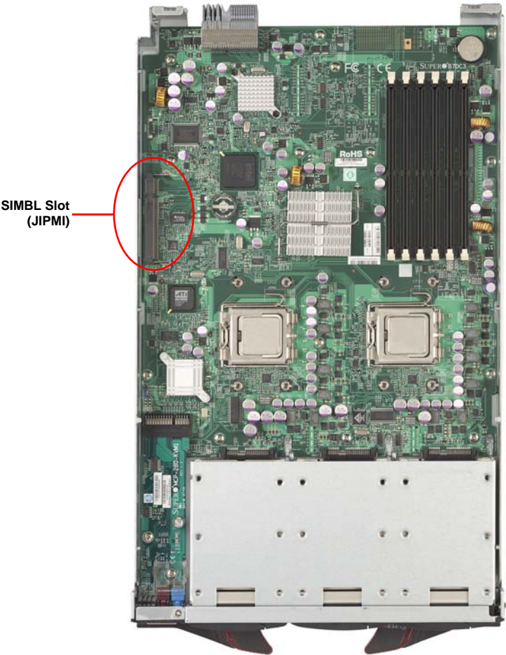
Figure 2-7. Location of SIMBL Slot on B7DC3 Motherboard
