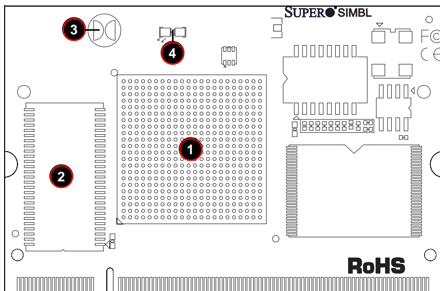
Figure 2-1. AOC-SIMBL Add-on Card – Front View
