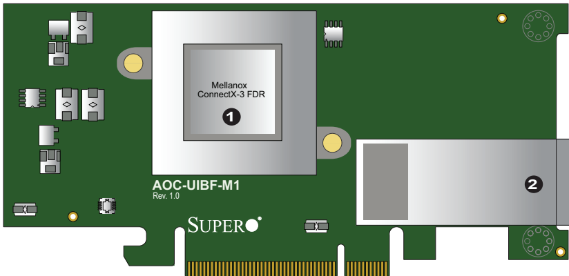
The AOC-UIBF-m1 Layout
