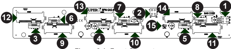
Figure 2-1: Front Connectors
