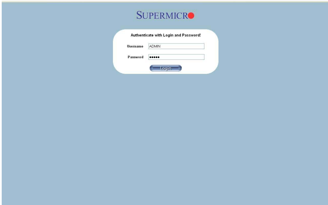
Fig 1: Login page
