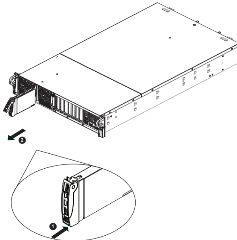
Figure 3-6. Removing a Drive Carrier
