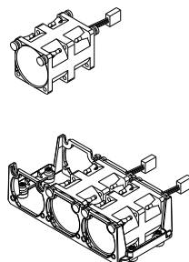
Figure 5-29: Removing the Fan from the Fan Tray
