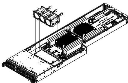
Figure 5-28: Removing the Fan Tray (Your node may differ slightly from the one shown in this illustration)
