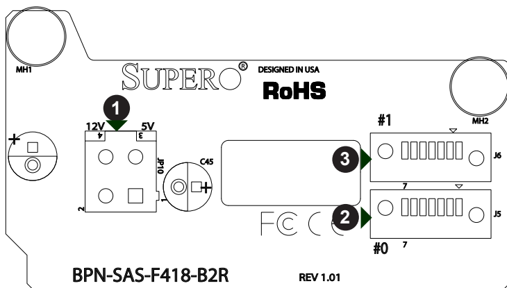
Figure C-1: Front Connectors
