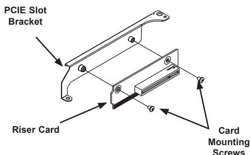
Figure 5-24: Assembling the PCIe Slot Bracket and Riser Card
