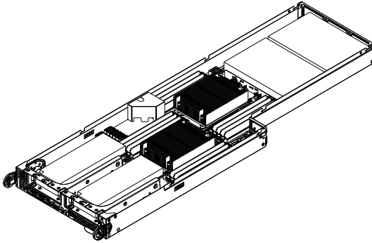
Figure 5-5: SCF418IF-R1K62BP Node
