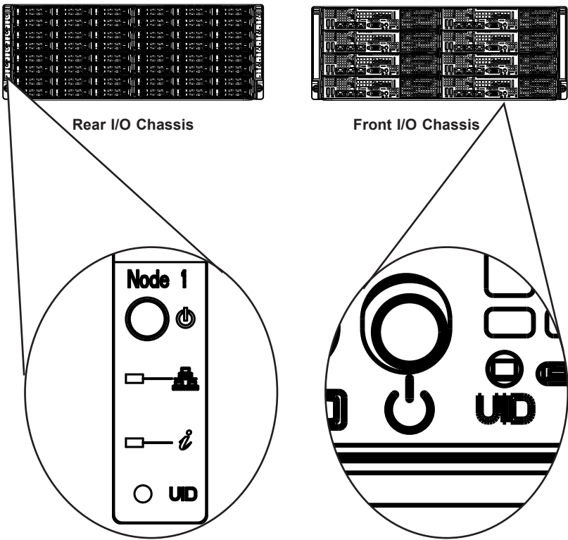
Figure 4-1: Chassis Control Panel
