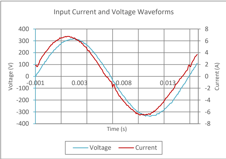
Input AC Current Waveform (ITHD = 3.62%, 50% Load)
