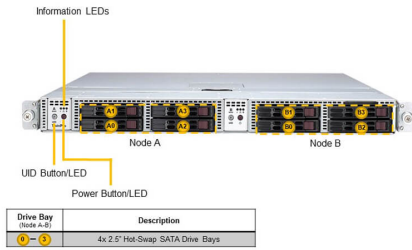
(Front View – System)
